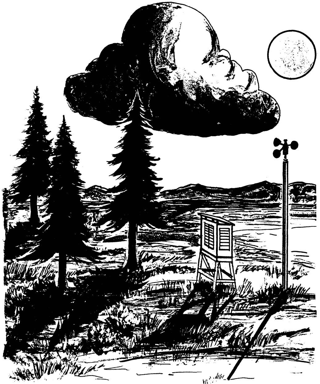
Figure 2.—Environmental conditions influencing fuels subject to solar heating are not measured by instruments in weather shelter.
