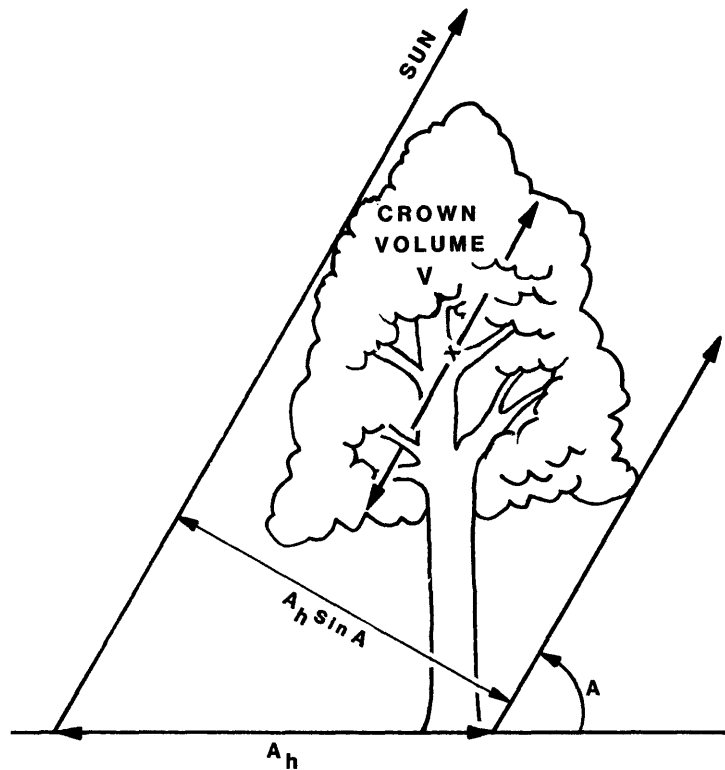
Figure 6C.—Intercrown path length relationship.
