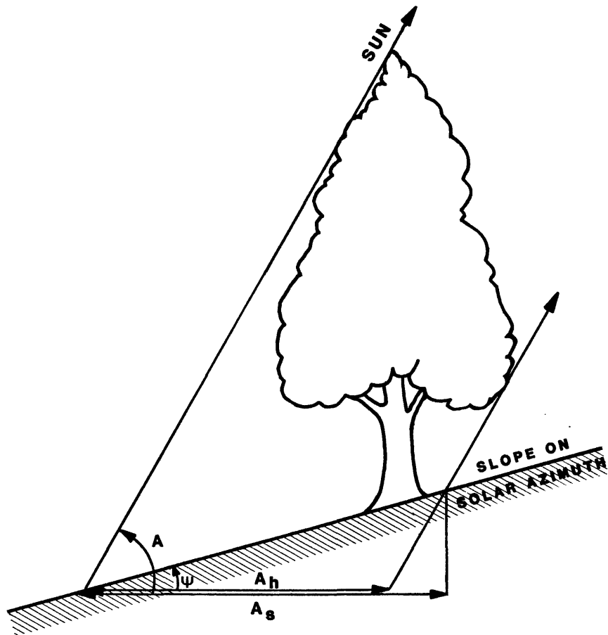
Figure 6D.—Shadow relationship to slope.
