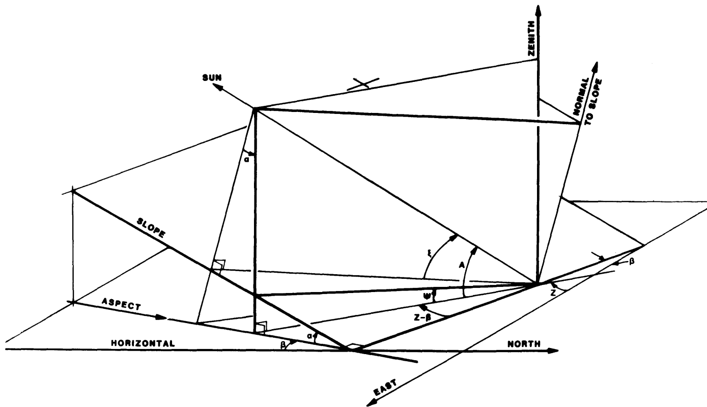
Figure 4.—Diagram of sun/slope geometry.
