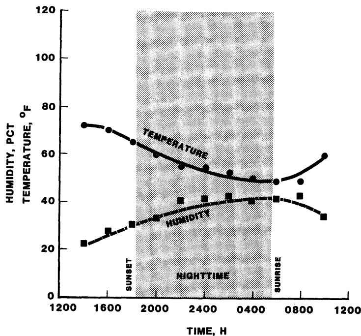
Figure 20.—Diurnal temperature and humidity measurements (dots and squares) and model predictions (lines) in Idaho in September beneath mixed conifer stand.
