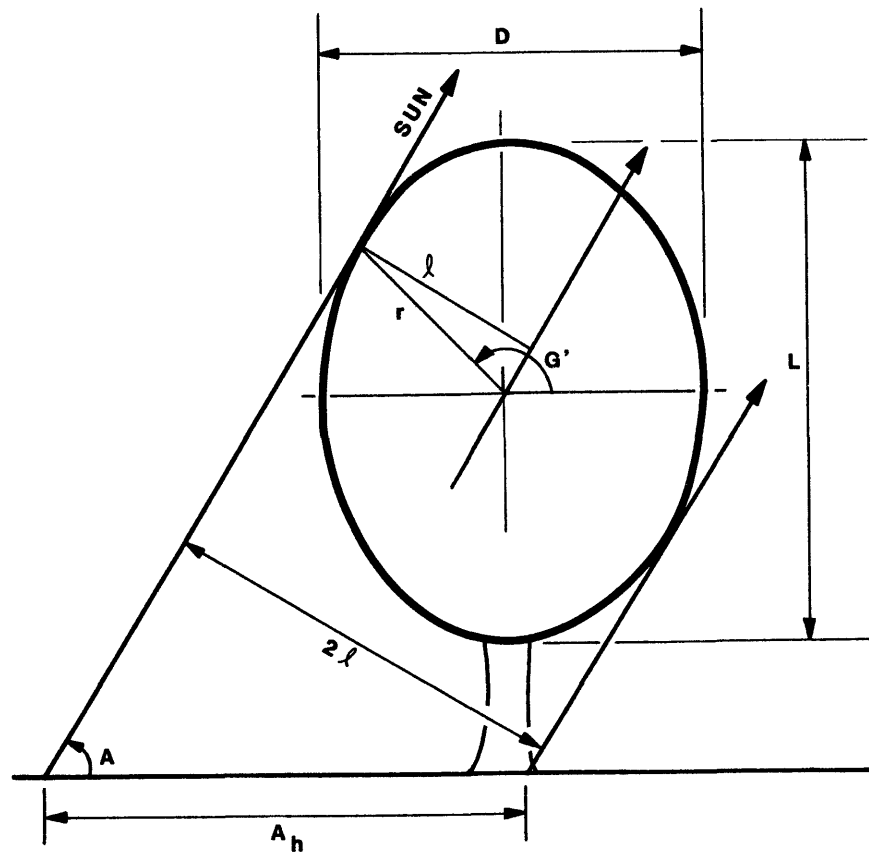
Figure 6B.—Deciduous tree shadow configuration.
